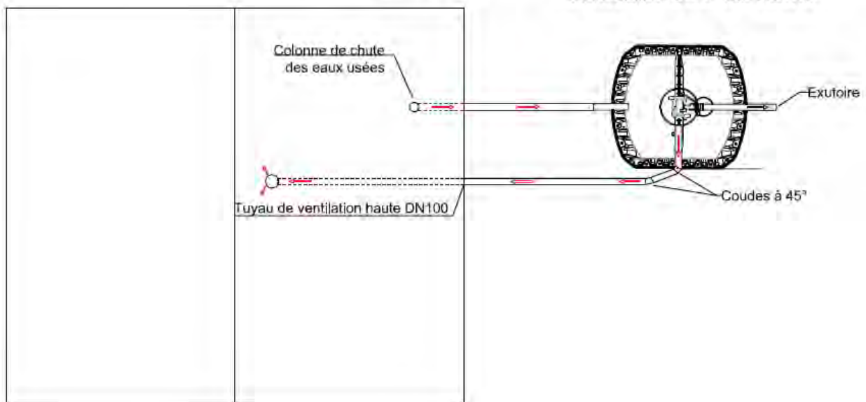
Illustration 10 : ventilation Quick
